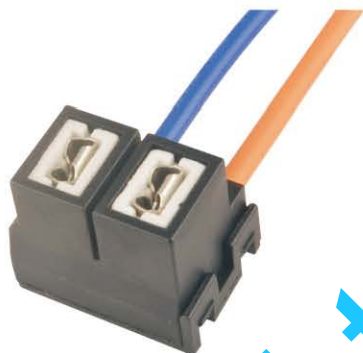
H7弯角陶瓷灯座 H7 bend angle ceramic lampholders
